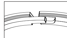
BRONZE INSERT RING - ONEP 2" to 48" 50.8mm to 1219.2mm
