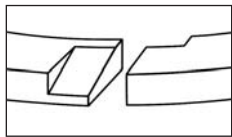
ANGLE STEP CUT 0.5" to 90" 12.7mm to 2286mm
