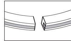
BRONZE INSERT RING - Butt Cut 2" to 48" 50.8mm to 1219.2mm
